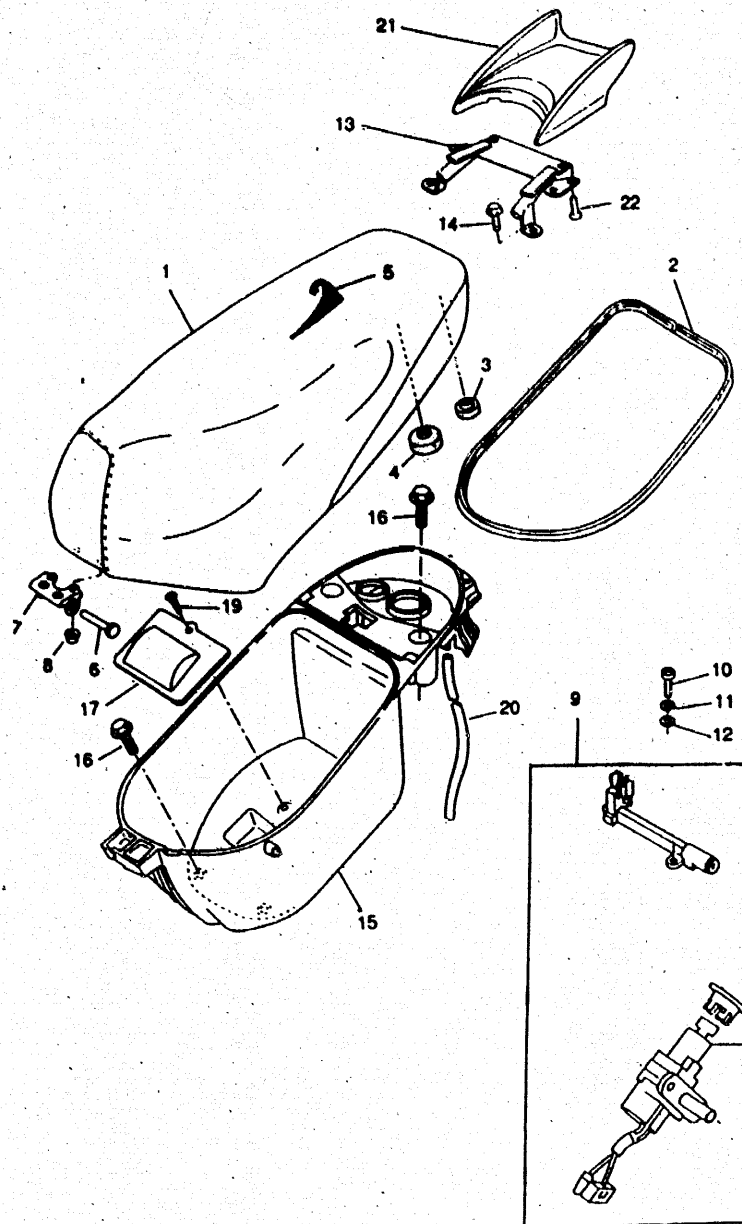
FIG 19 SEAT. CARRIER
