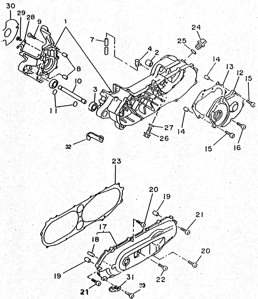
FIG 8 CRANKCASE
