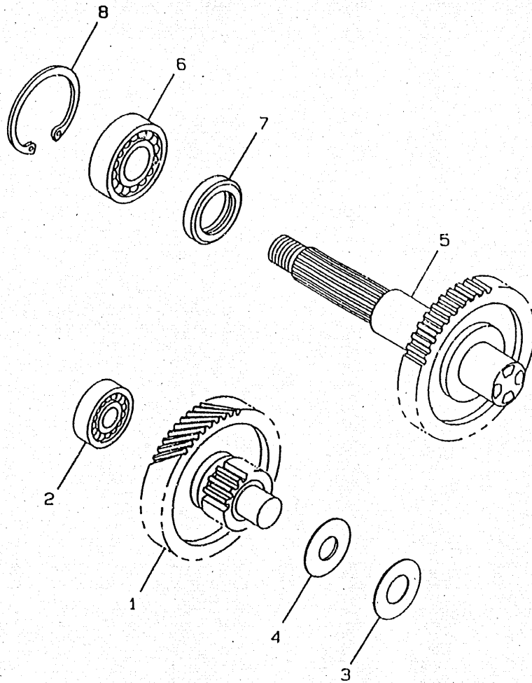
FIG 11 TRANSMISSION
