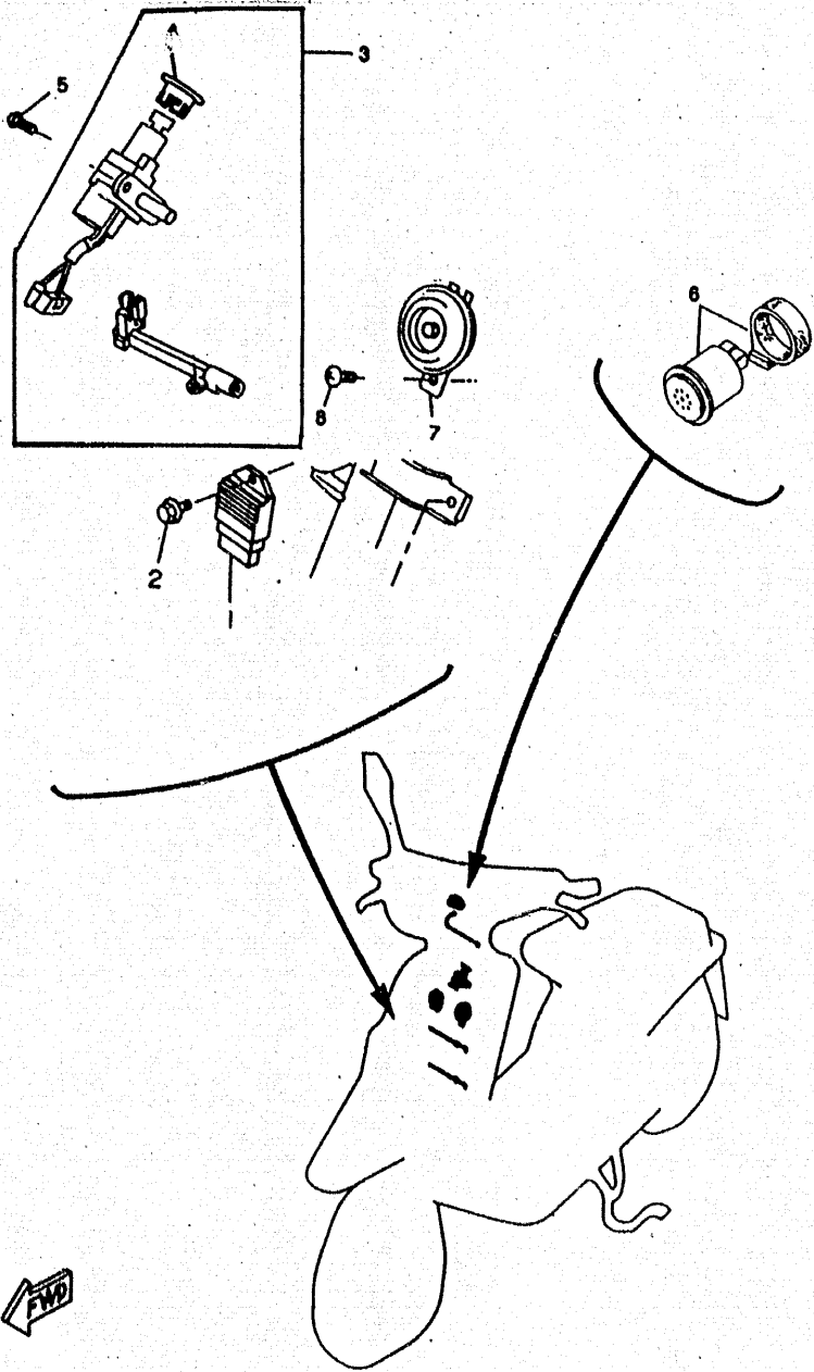
FIG 34 ELECTRICAL1
