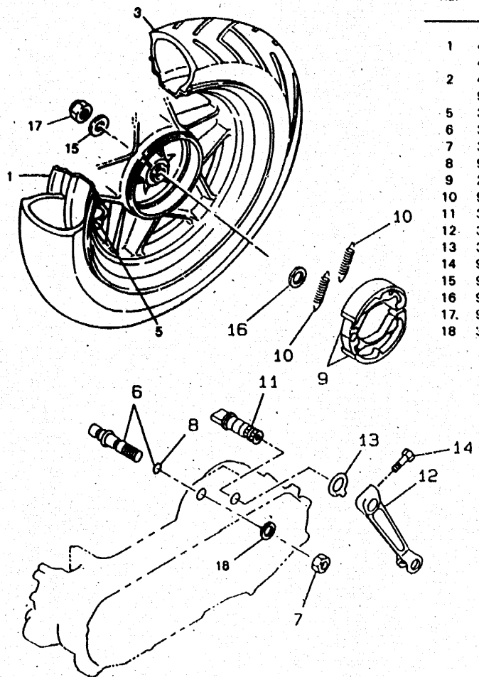
FIG 22 REAR WHEEL
