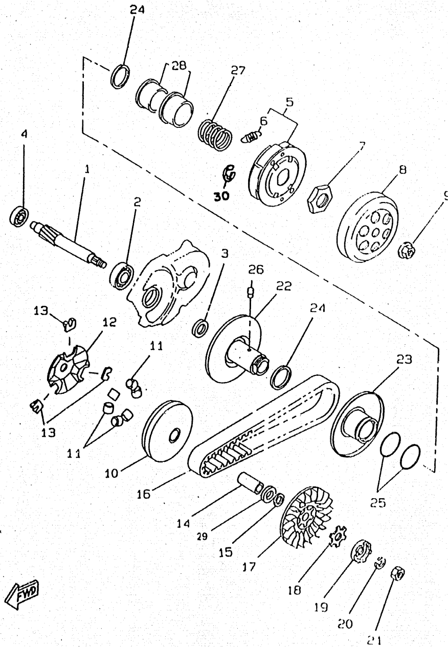
FIG 10 CLUTCH
