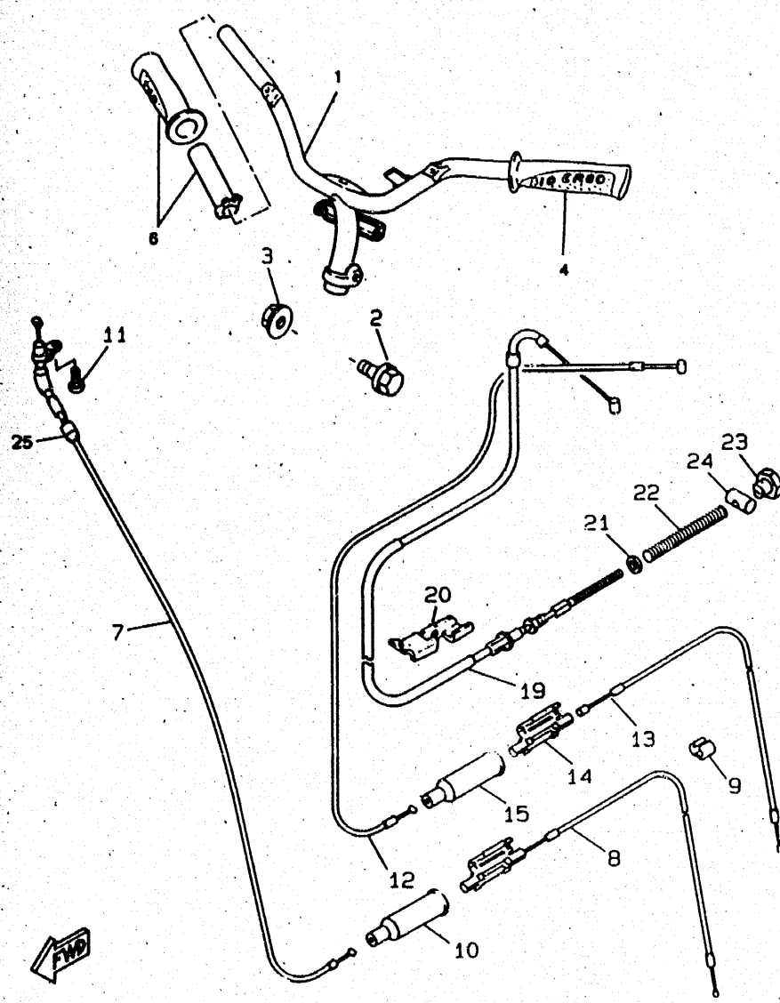
FIG 23 STEERING HANDLE. CABLE
