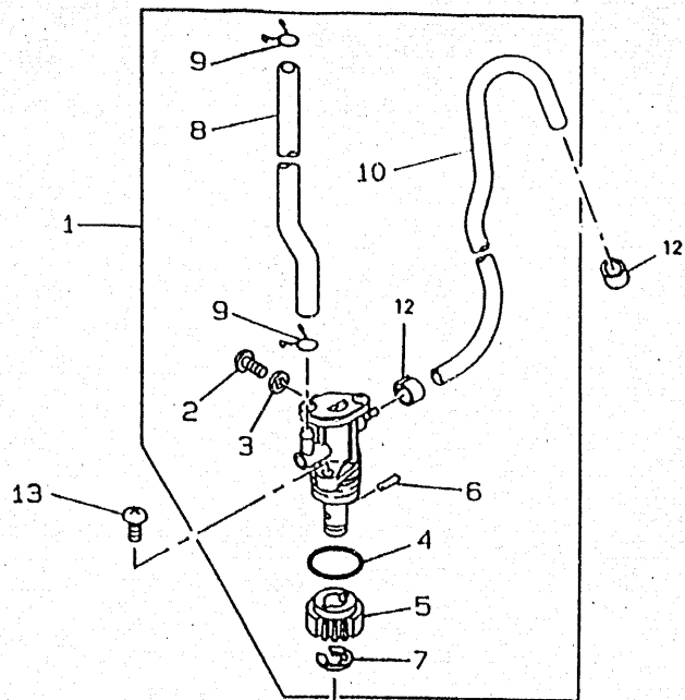
FIG 4 OIL PUMP
