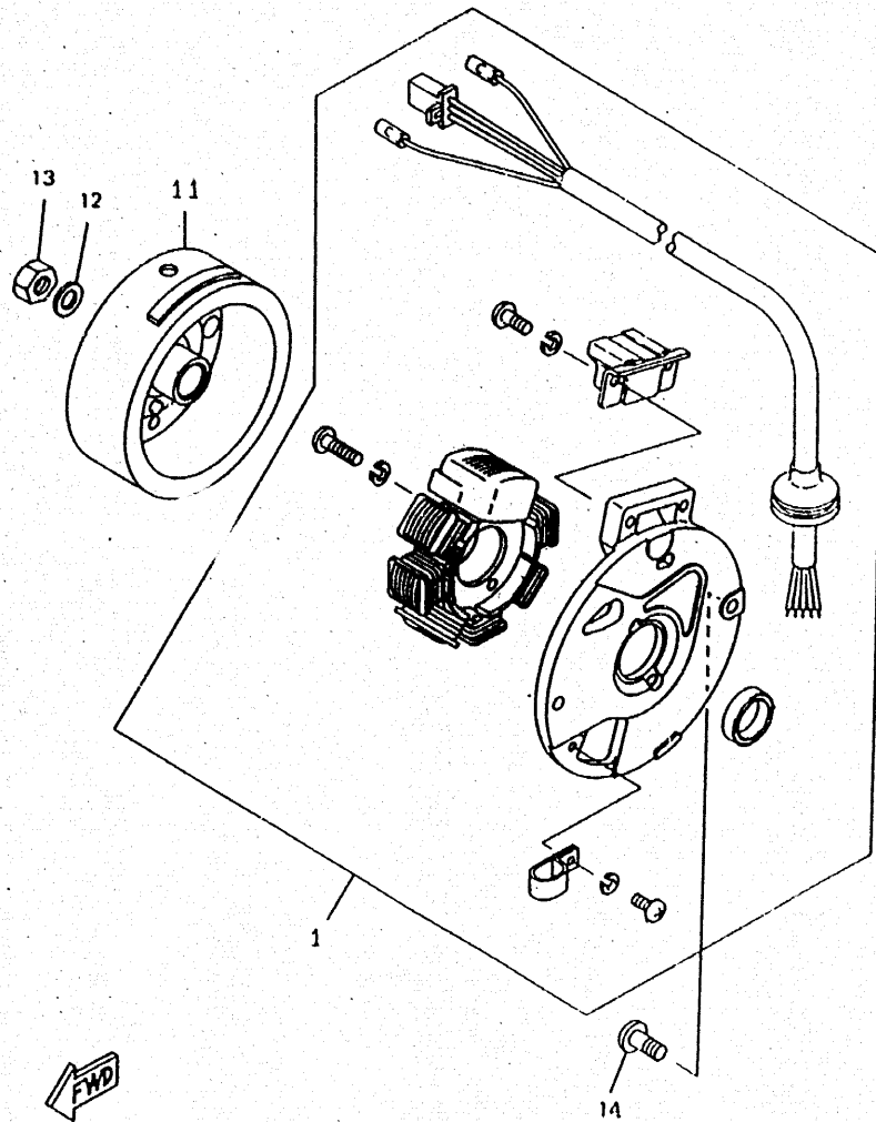
FIG 28 GENERATOR
