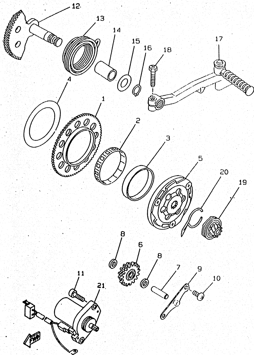
FIG 9 STARTER
