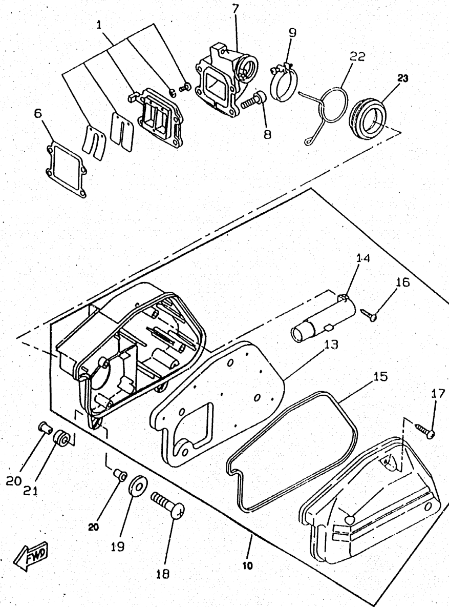
FIG 5 INTAKE
